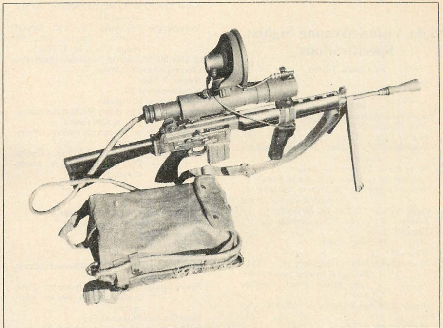
Representative infrared unit mounted on Armalite AR-18. Note IR light source mounted over telescope, special flash-hider. Backpack contains 6-volt ni-cad battery and power-pack to convert to 20,000 volts required to run electronic telescope. Has continuous-use life of 20 hrs. before recharging is required. Special ni-cad battery can be recharged 5000 times before replacement.
